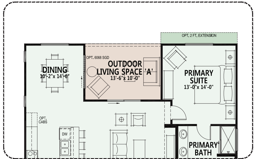
Opt. Dining Extension
