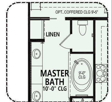
Opt. Pocket Door at Master Bath
