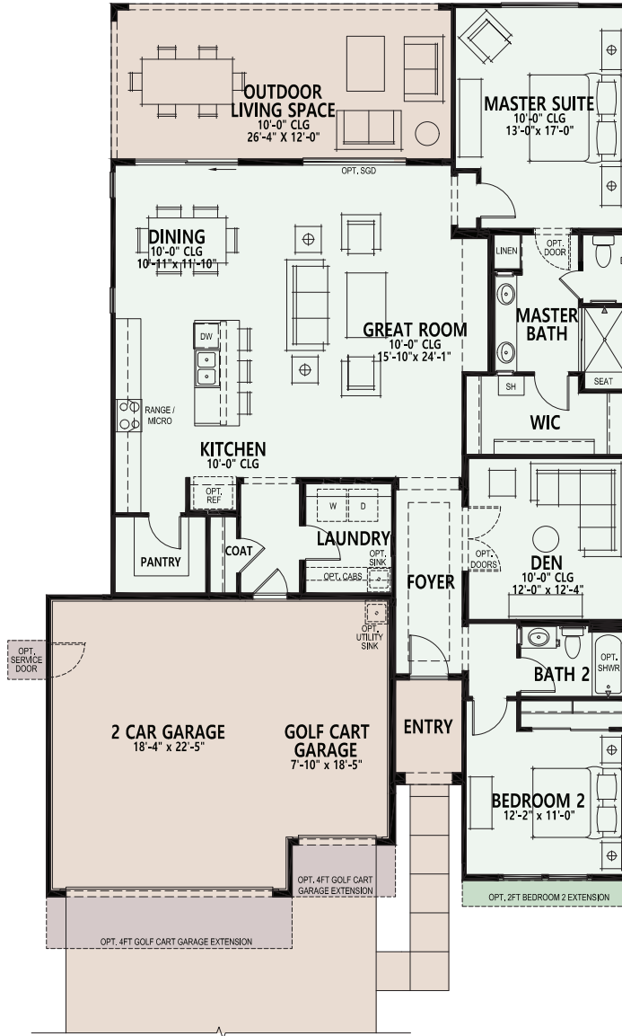
Opt. 2 ft Great Room, Outdoor Living Space and Laundry Extension w/ Golf Cart Garage
