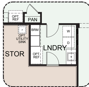
Opt FF Cabs w/ Broom Closet and Ref Space at Laundry
